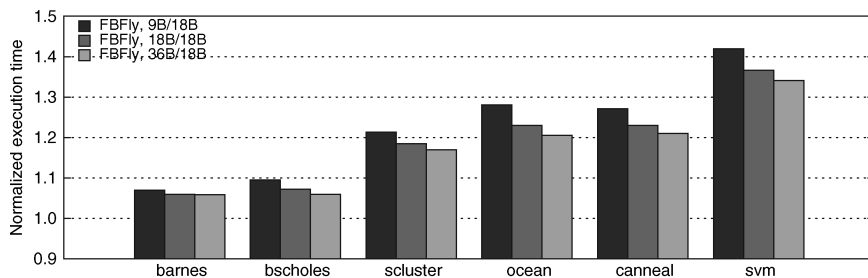
(a) Performance with varying local flit size.
