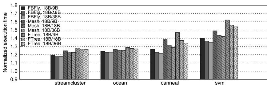
(b) Performance with varying global flit size.
