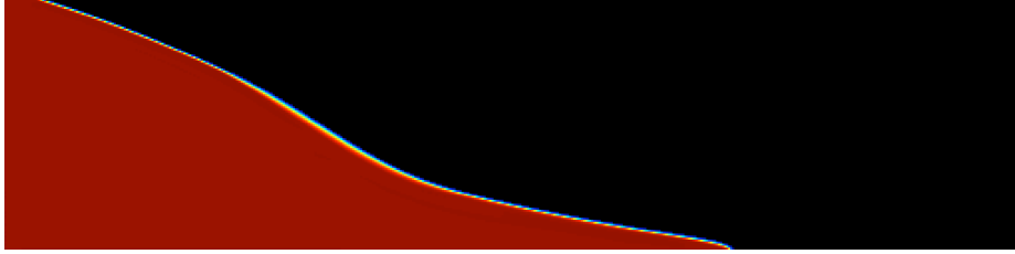
Figure 1. Solution of n_1 at 8 \times 10^6 s.
