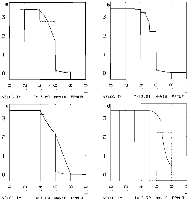
FIG. 5. A single time step in the computation of a strong shock using the PPM scheme. Velocities are displayed for 5 zones representing various stages in the computation. See the discussion in Section Vc of the text. (a) Interpolation parabolae (solid lines) are constructed from the original zone-averaged data (dotted lines). The shock is only one zone wide. (b) Data are obtained for Riemann problems which will give time-averaged fluxes at zone interfaces in a Lagrangian step of the calculation. The data (solid lines) are obtained by averaging the interpolation parabolae (dotted lines) over the domains of dependence of each zone interface. (c) The solution of the Riemann problems (represented by dotted lines) gives effective velocity gradients within the zones (solid lines) which compress the Lagrangian zones. (d) The compressed Lagrangian zones are shown by solid lines with internal structures inferred from zone-averaged data by the construction of new interpolation parabolae. New averages are computed using these parabolae for the original Eulerian zones (dotted lines). The shock has moved \frac{3}{4} of a zone width and is again only one zone wide.
